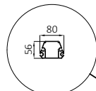
ALM.PRF.P1030 Fabric Support Profile (Double)
