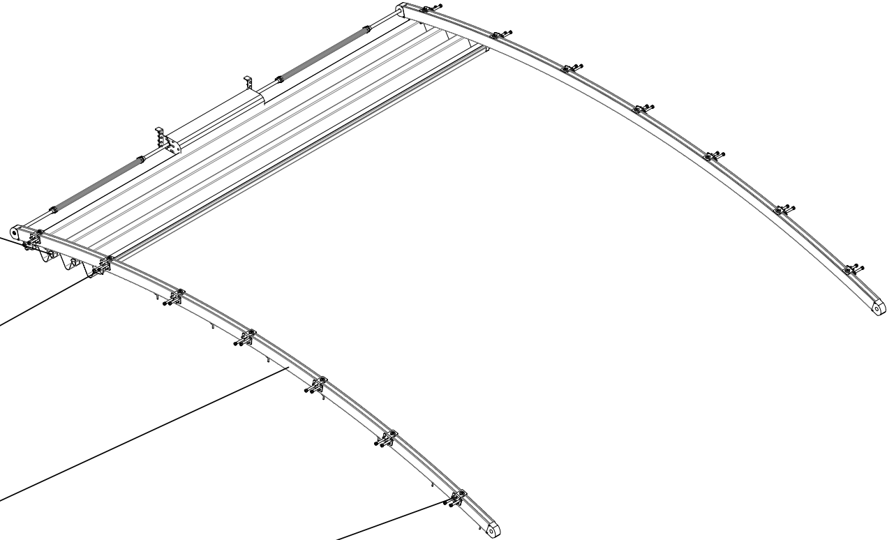
ALM.PRF.P1026 Fabric Support Profile (Single)
