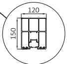
ALM.PRF.P1008 Rail Profile
