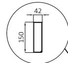
ALM.PRF.G1012 Motor Fixing Beam
