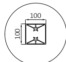
ALM.PRF.G1001 Back Pillar
