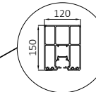
ALM.PRF.P1009 Rail Profile (8-10m)
