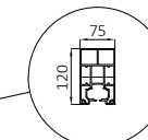
ALM.PRF.P1018 Rail Profile
