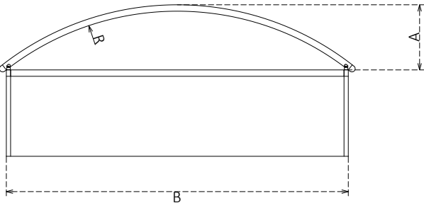
RADIUS CHART
