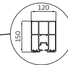
ALM.PRF.P1008 Rail Profile
