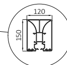
ALM.PR.F.P1003 Rail Profile
