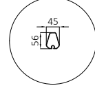
ALM.PRF.P1026 Fabric Support Profile (Single)
