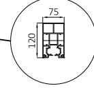
ALM.PRF.P1021 Rail Profile
