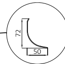
ALM.PRF.G1011 Wall Finish
