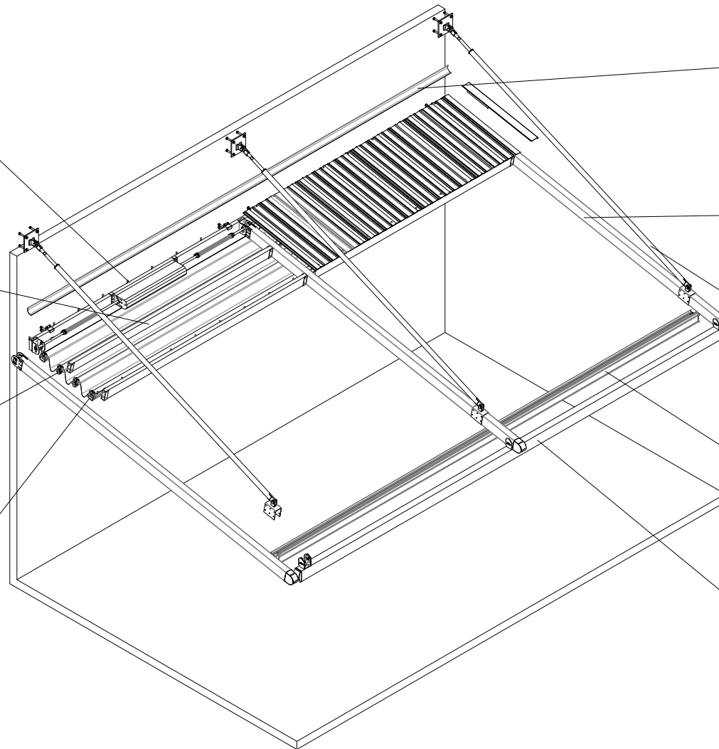
ALM.PRF.P1026 Fabric Support Profile (Single)
