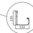
ALM.PRF.P1007 Gutter
