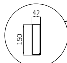
ALM.PRF.G1012 Front Cross Beam
