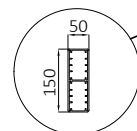
ALM.PRF.G1009 Side Beam
