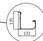
ALM.PRF.P1007 Gutter
