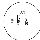
ALM.PRF.P1030 Fabric Support Profile (Double)
