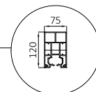
ALM.PRF.P1018 Rail Profile
