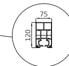
ALM.PRF.P1021 Rail Profile
