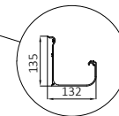
ALM.PRF.P1007 Gutter
