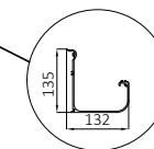
ALM.PRF.P1007 Gutter
