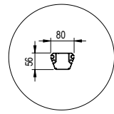
ALM.PRF.P1001 Aluminum fabric profile | Double channeled
