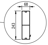
ALM.PRF.G1066 Support Box Profile
