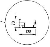
ALM.PRF.G1058 Gutter Profile
