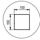
ALM.PRF.G4033 Aluminum pillar profile | 150x150mm
