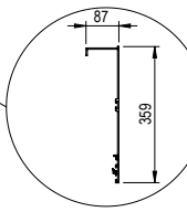
ALM.PRF.G1059 Face Profile
