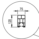
ALM.PRF.P1018 Aluminum Rail Profile
