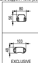
Fabric Support Profile (Double)
