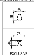
Fabric Support Profile (Single)
