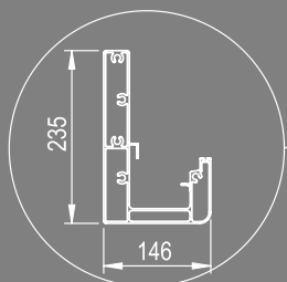
Integrated Beam
