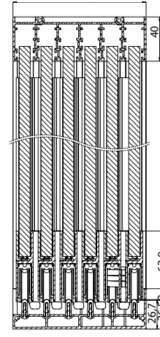
6 Railed Sliding System S
