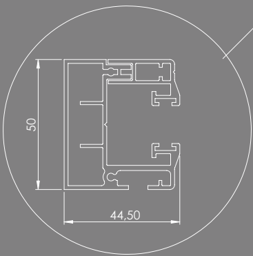
Rail Profile
