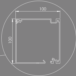
Cassette Profile
