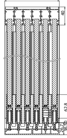
6 Railed Sliding System S
