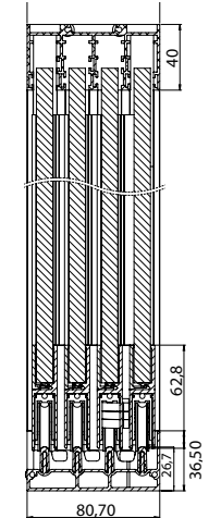
4 Railed Sliding System S
