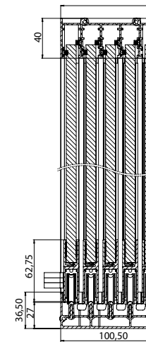
5 Railed Sliding System S
